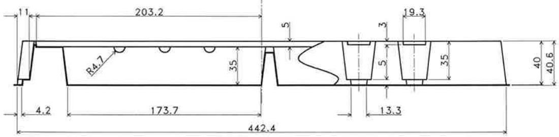
SECTION "X-X"
