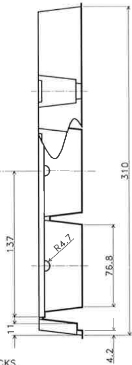
SECTION "Y-Y"
