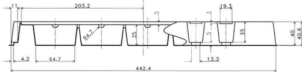
SECTION "X-X"
