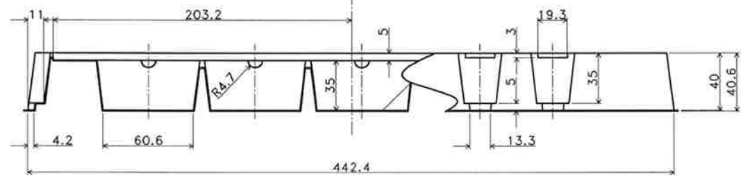
SECTION "X-X"
