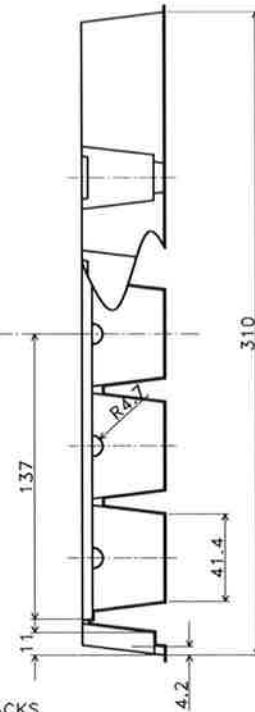
SECTION "Y-Y"
