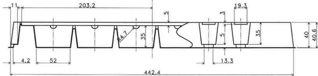
SECTION "X-X"
