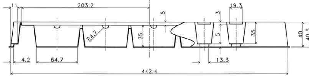
SECTION "X-X"
