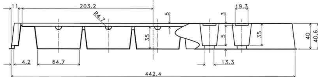
SECTION "X-X"
