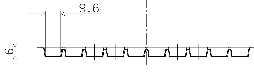
SECTION "X-X"
